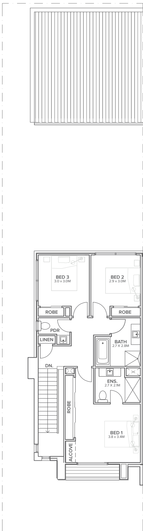
FIRST FLOOR
