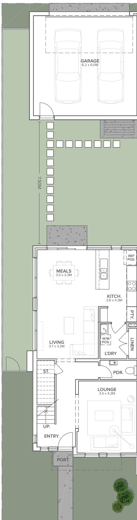
GROUND FLOOR
