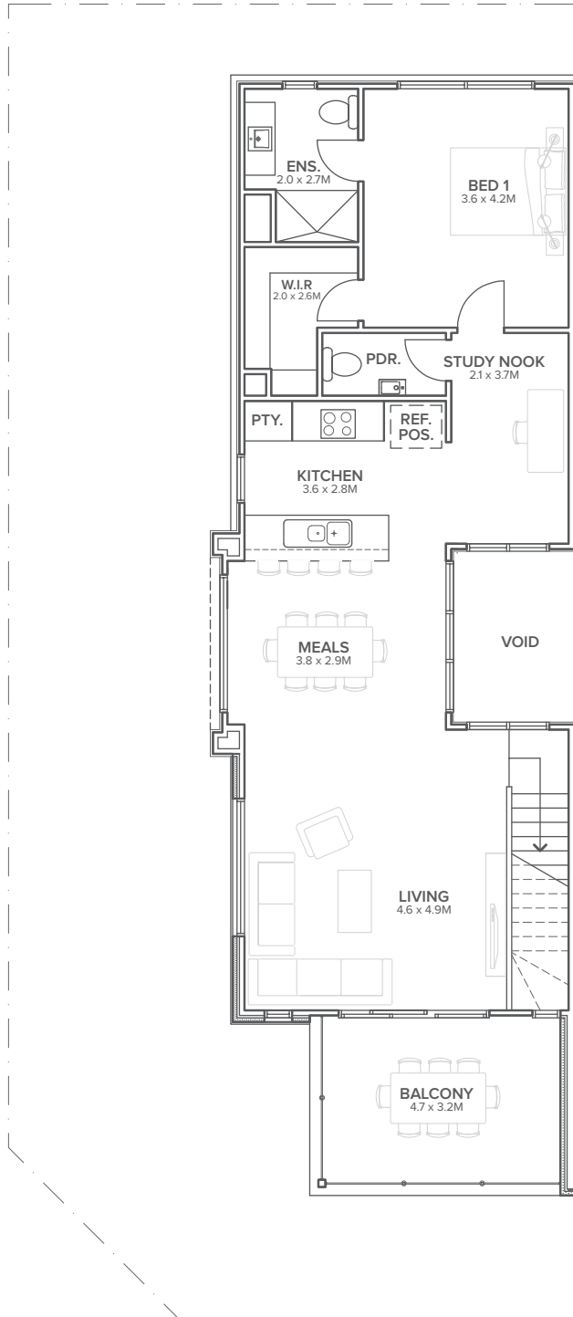
FIRST FLOOR
